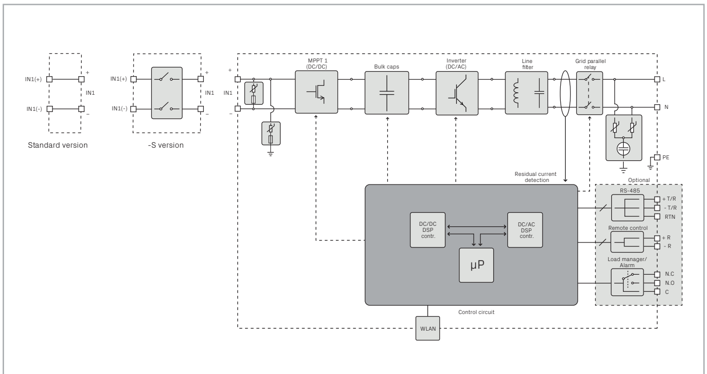
UNO-DM-1.2/2.0/3.0-TL-PLUS string inverter block diagram
