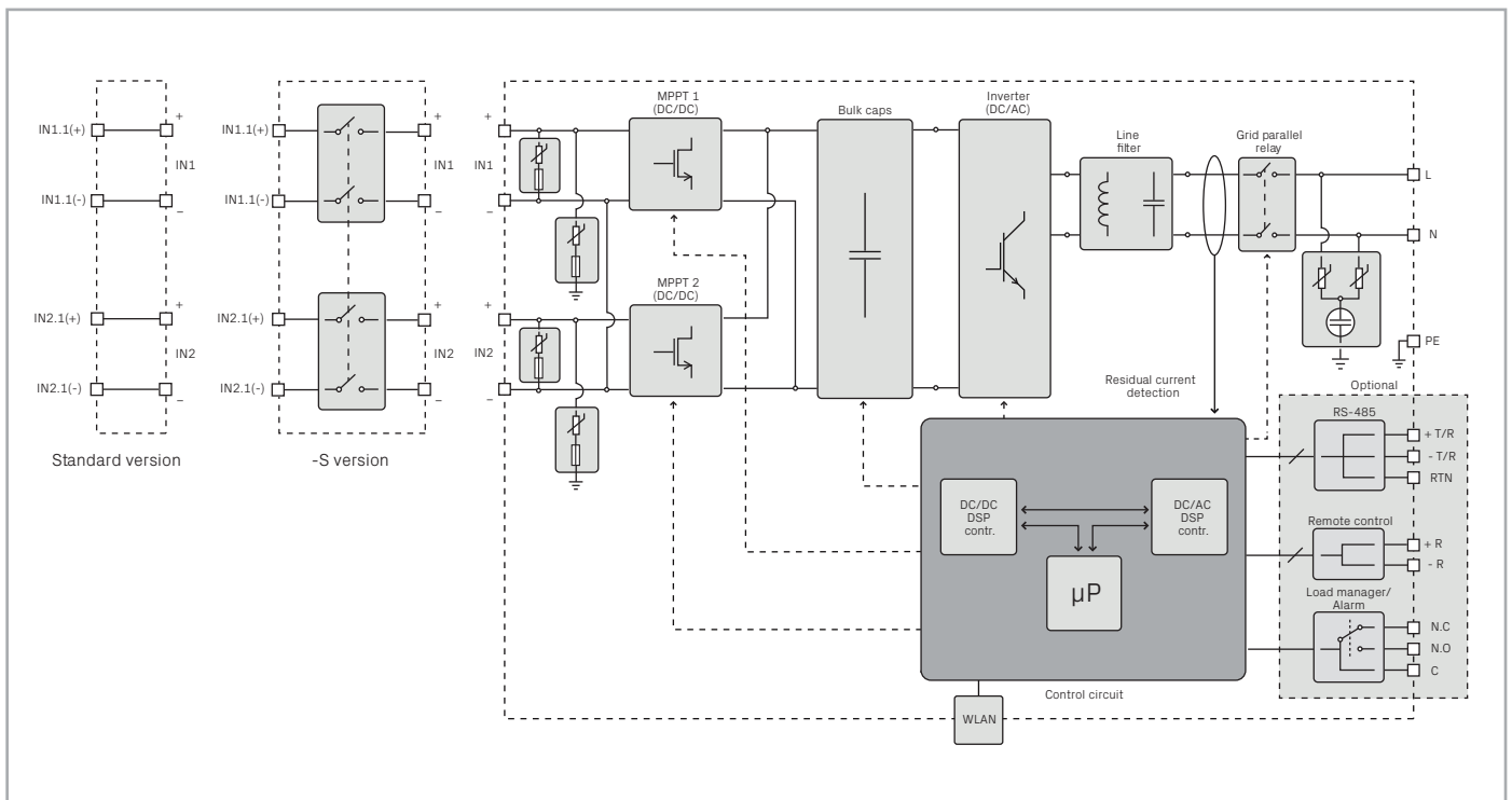
UNO-DM-6.0-TL-PLUS string inverter block diagram
