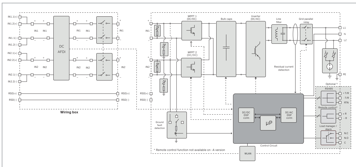
UNO-DM-3.3/3.8/4.6/5.0-TL-PLUS-US string inverter block diagram
